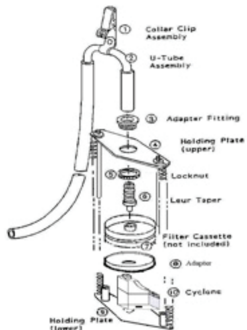
▲ The sampling train of virtual cyclone for respirable dusts
